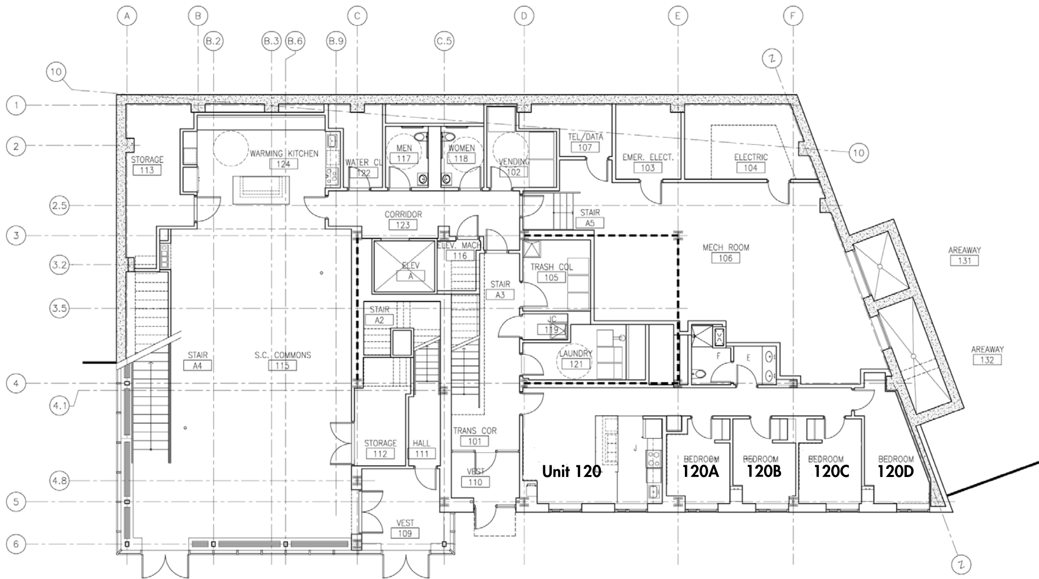
Building A: First Floor
