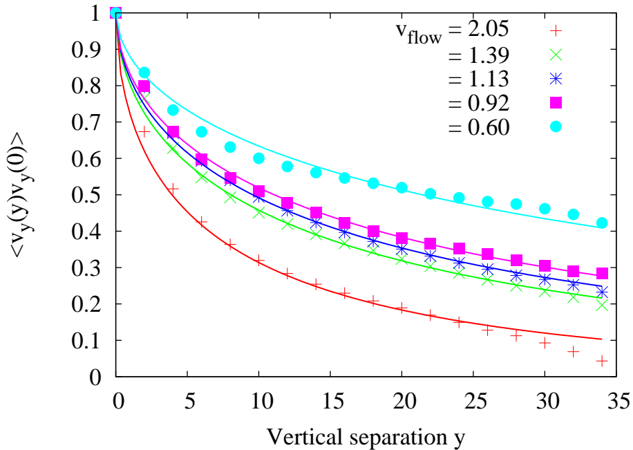
FIG. 8: (Color online) The equal time spatial correlation function of the vertical velocity component is shown as a function of vertical separation at five different flow rates. The points are obtained from the numerical simulation, and the solid lines represent fits to the data using the stretched exponential function \exp[-(x/\lambda)^{0.55}] with \lambda as the only fitting parameter.
