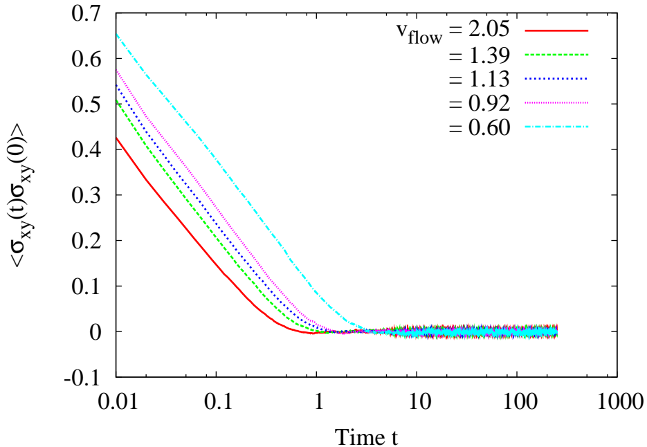
FIG. 6: (Color online) Autocorrelation of the shear stress at the same five flow rates.
