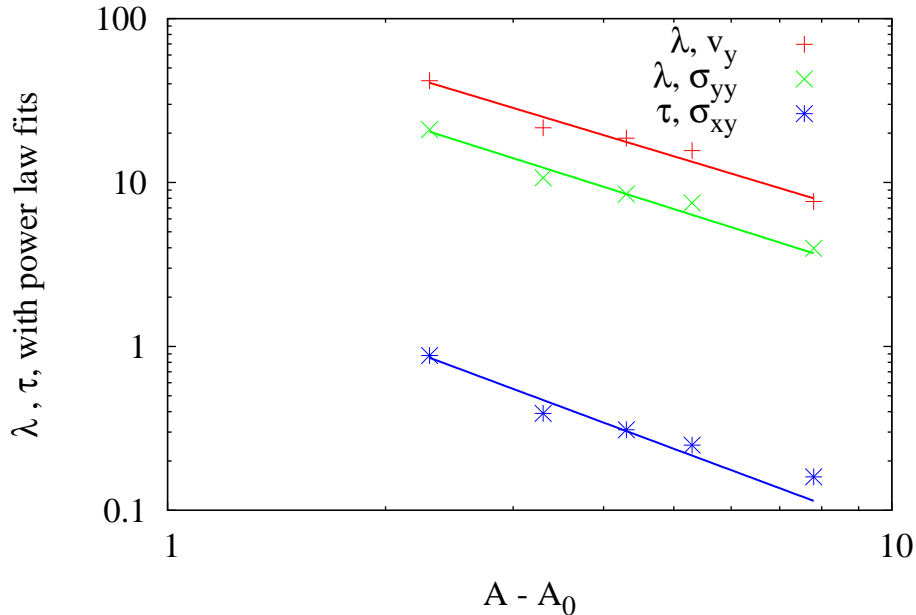
FIG. 13: (Color online) The length scales \lambda obtained from the equal time spatial correlation functions of v_y and \sigma_{yy} and the timescale \tau from the autocorrelation of \sigma_{xy} are plotted as a function A - A_0 , where A is the size of the opening, and A_0 the opening at which the flow velocity extrapolates to zero. The solid lines are power law fits with exponents -1.3 ( \lambda, v_y ), -1.4 ( \lambda, \sigma_{yy} ), and -1.6 ( \tau, \sigma_{xy} ).
