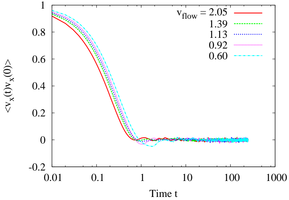
FIG. 4: (Color online) Autocorrelation of the velocity component perpendicular to the flow at five different flow rates. The flow rates are expressed in units of particle diameters per simulation time.
