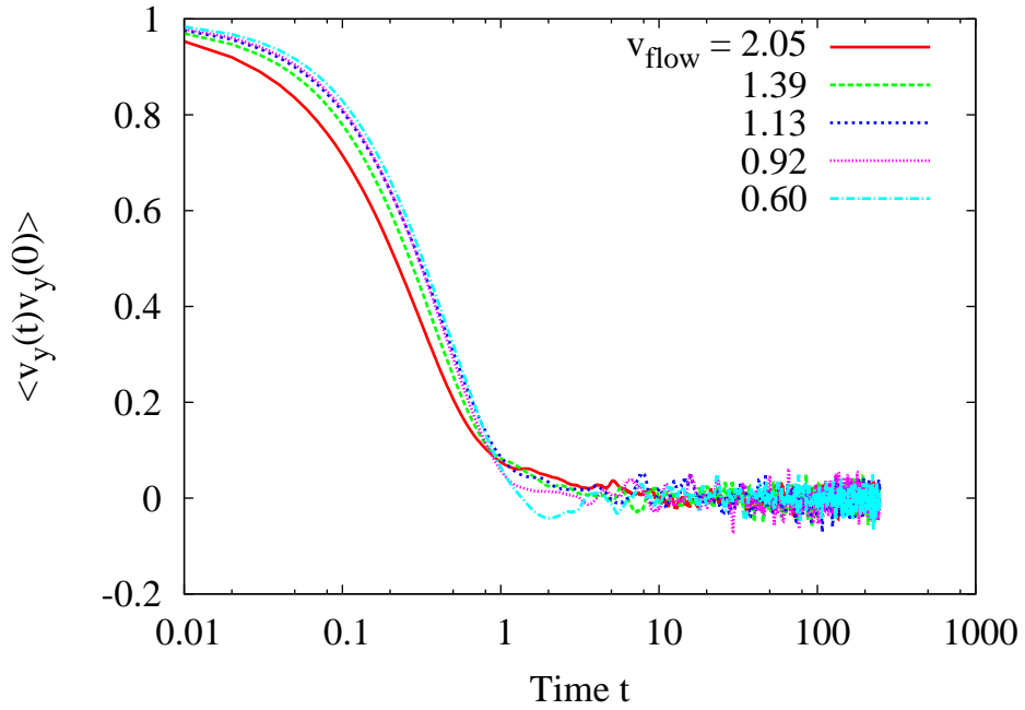
FIG. 5: (Color online) Autocorrelation of the velocity component parallel to the flow at the same five flow rates.
