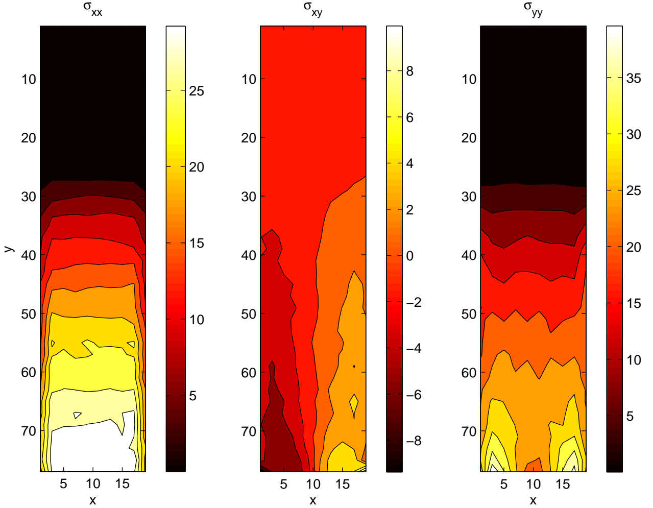
FIG. 2: (Color online) Contour plots (a) - (c) of the time-averaged profiles of the stress tensor components \sigma_{xx} (horizontal pressure), \sigma_{xy} (shear stress) and \sigma_{yy} (vertical pressure) respectively.
