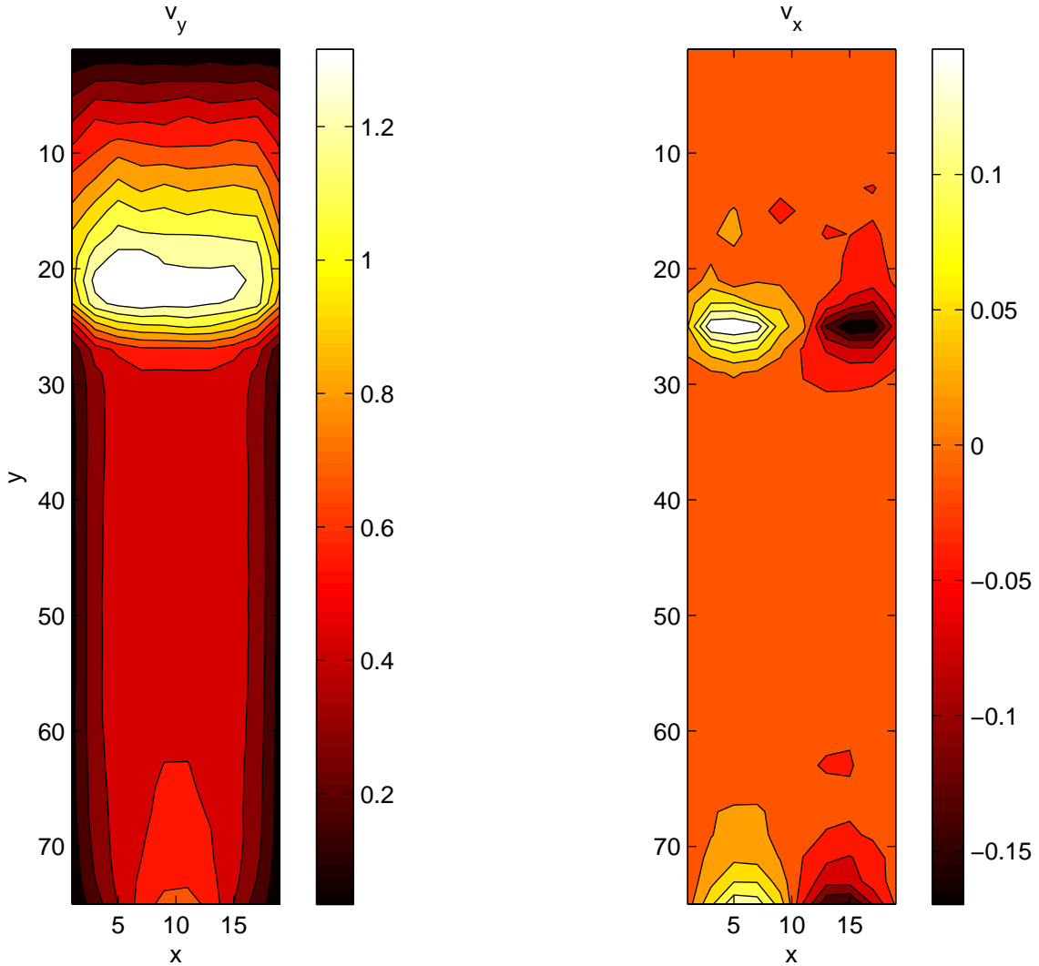
FIG. 1: (Color online) Contour plot of the time-averaged spatial profile of the velocity components. (a) shows the component parallel to the flow, and (b) shows the component of velocity perpendicular to the flow. We focus on the region where the velocity remains approximately constant.
