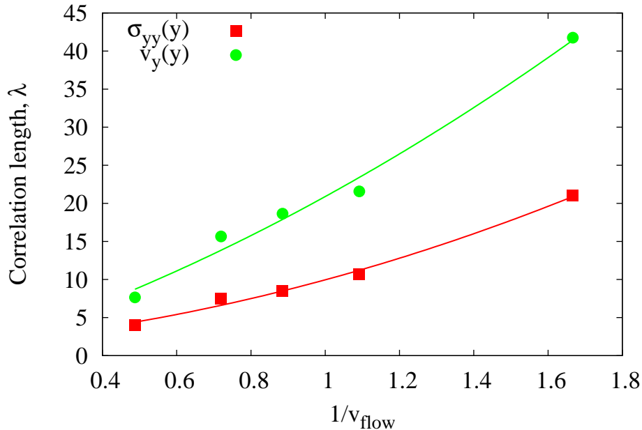
FIG. 11: (Color online) The length scales \lambda obtained from fitting the equal time spatial correlation functions \langle v_y(y)v_y(0) \rangle and \langle \sigma_{yy}(y)\sigma_{yy}(0) \rangle to a stretched exponential decay \exp[-(x/\lambda)^{0.55}] are plotted as a function of inverse flow rate.
