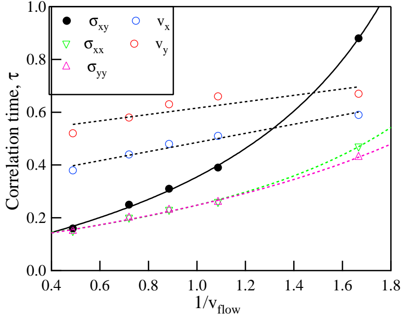
FIG. 7: (Color online) Time at which the autocorrelations of the different velocity and stress components drop to 0.1 as a function of the inverse flow velocity. The lines are intended as guides to the eye and are obtained from quadratic fits to the data. Note the timescale associated with the shear stress shows a much greater dependence on flow velocity.
