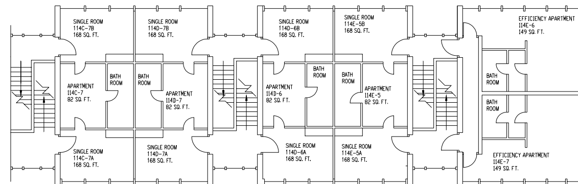
FIFTH FLOOR
