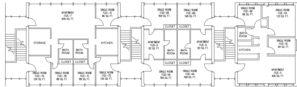
FOURTH FLOOR
