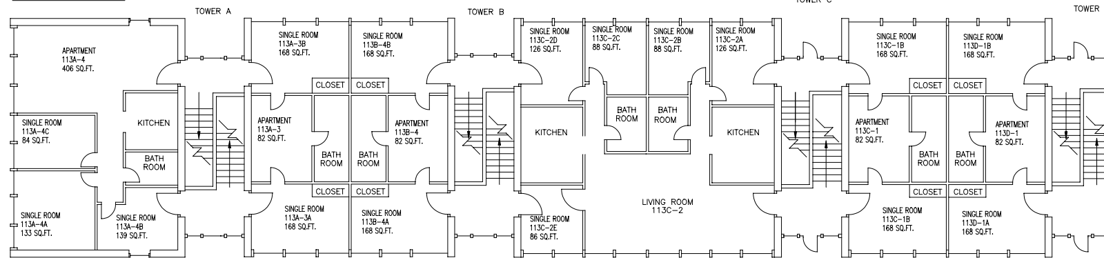
SECOND FLOOR
