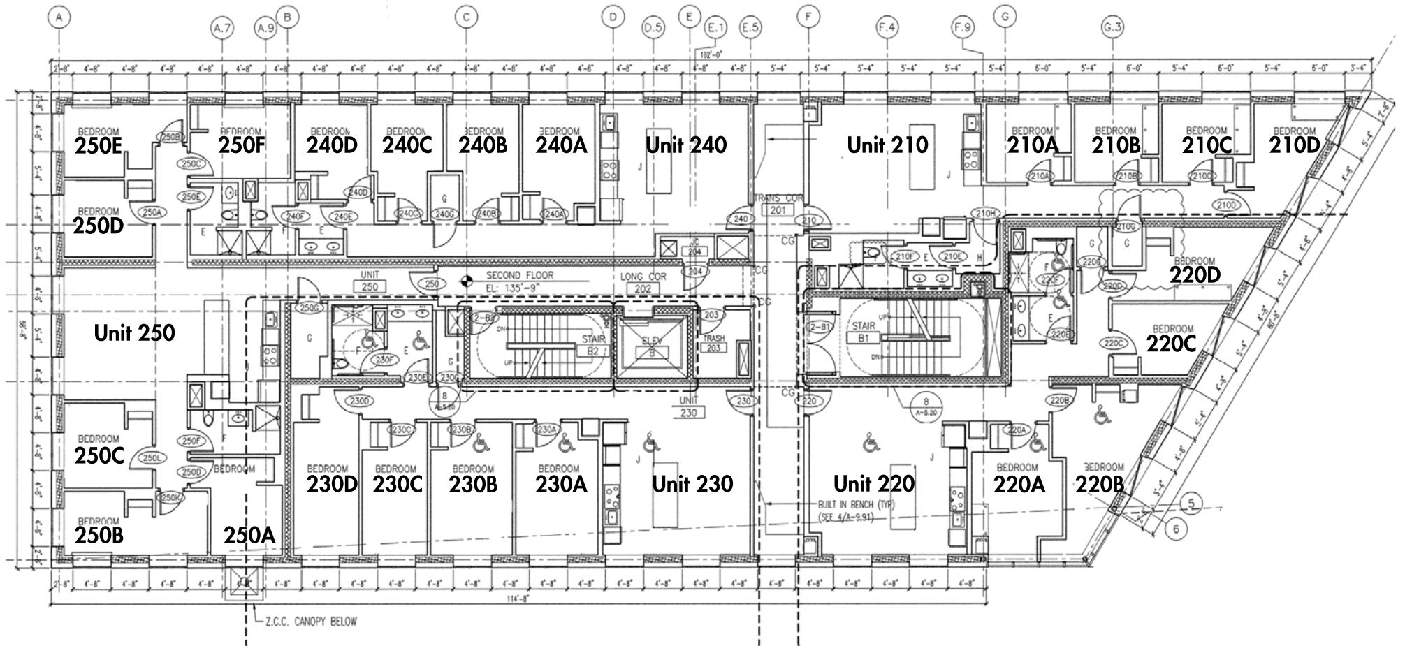
Building B: Second Floor
