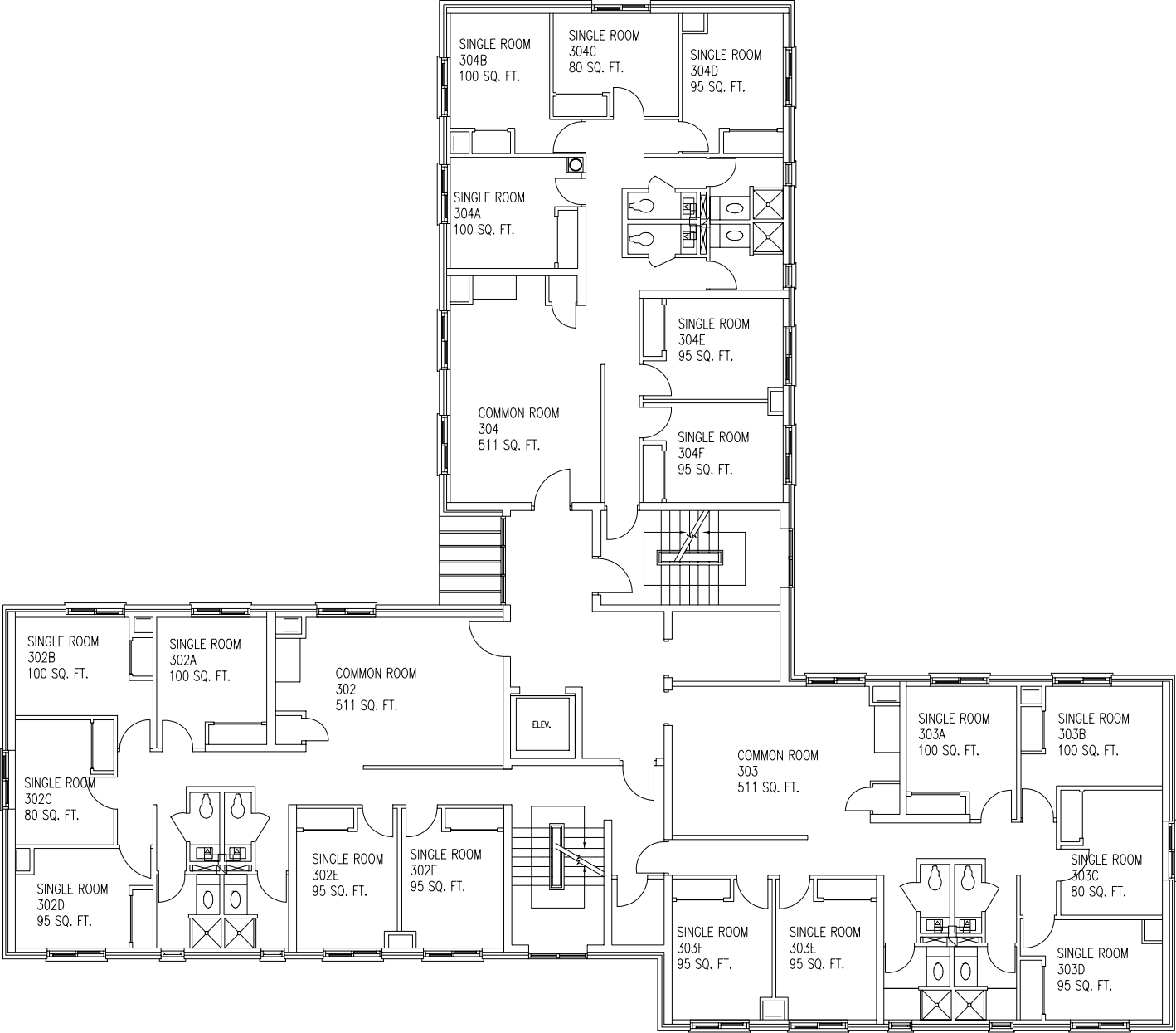
THIRD FLOOR
