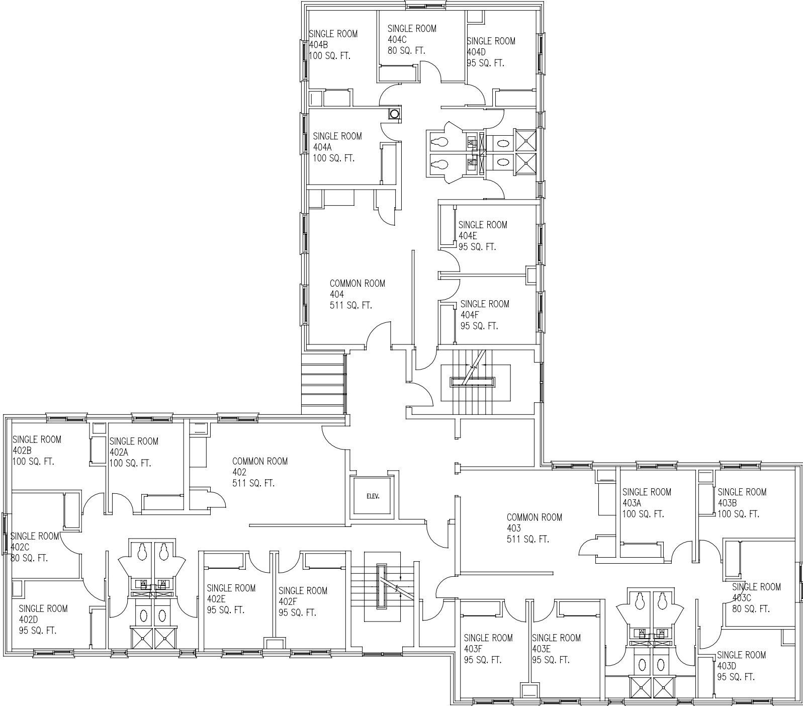
FOURTH FLOOR
