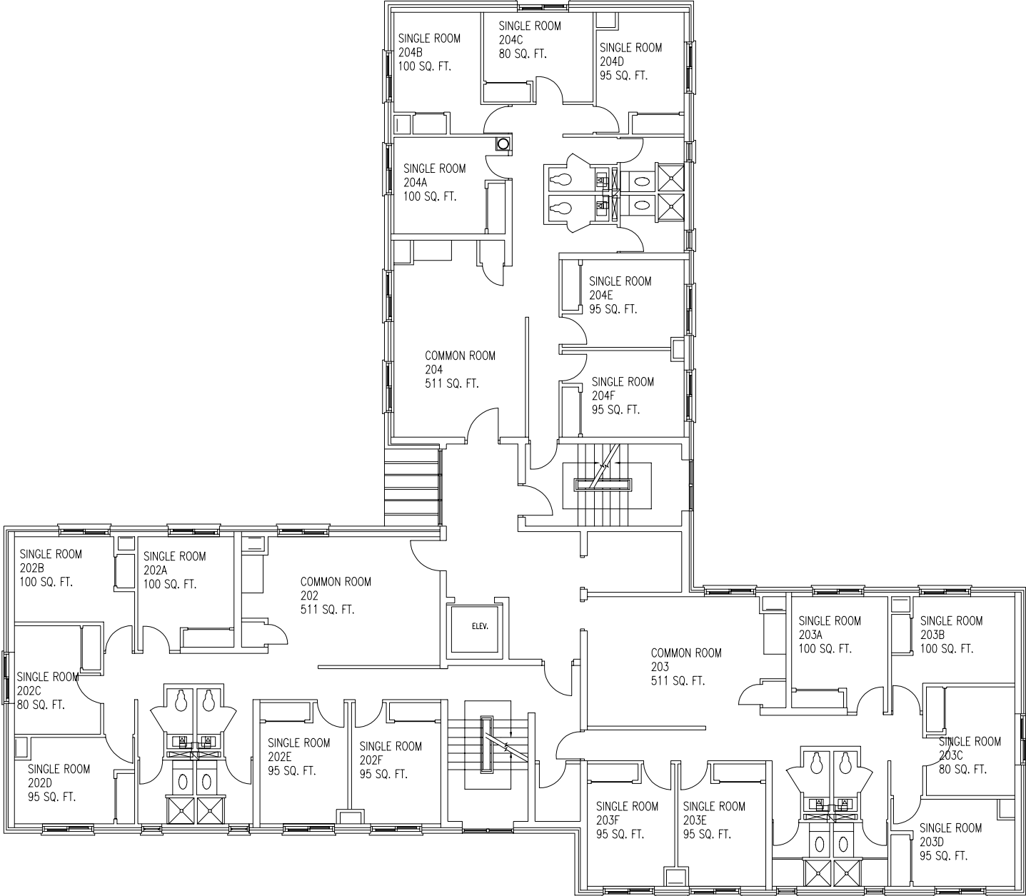
SECOND FLOOR
