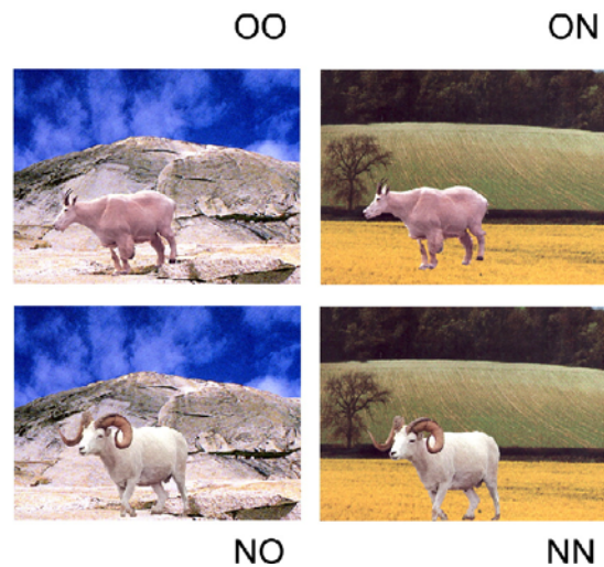
Fig. 1. Example recognition picture stimuli. Each picture consists of an object placed on a meaningful background. At recognition, the object and background independently can be either old, that is, identical to one presented at encoding, or new. The object's classification as either Old or New is denoted by the first letter in each condition name, and the background's classification is denoted by the second letter (e.g., a novel object on a previously studied background is denoted NO).
